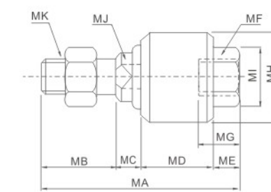
M-UJ Type Float Joint
