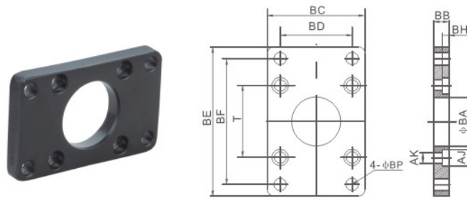
FA/FB Type Flange
